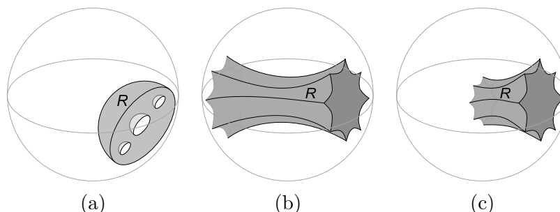
Figure 1: A typical fundamental domain R of (a) a handlebody, (b) a class A manifold with two boundaries, and (c) a non-handlebody with one boundary, in the hyperbolic 3-space \mathbf{H}_3 .
