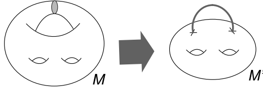
Figure 2: Reducing M to M' along a filled handle.
